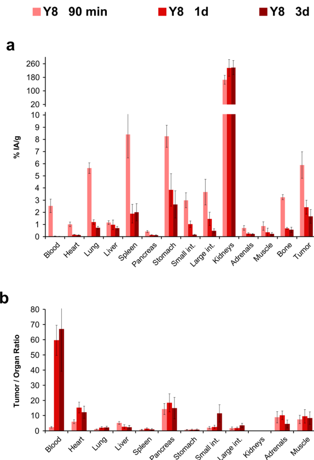
Fig. 5 Biodistribution in H209 tumor mice, and resulting tumor-to-organ ratios for the ^{177}\text{Lu} -labeled tetramer Y8 at different time points after injection. For details and numerical data in tabular form, see ESI.†
