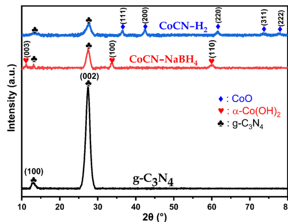
Fig. 3 XRD patterns of \text{CoCN-H}_2 , \text{CoCN-NaBH}_4 , and g\text{-C}_3\text{N}_4 .
