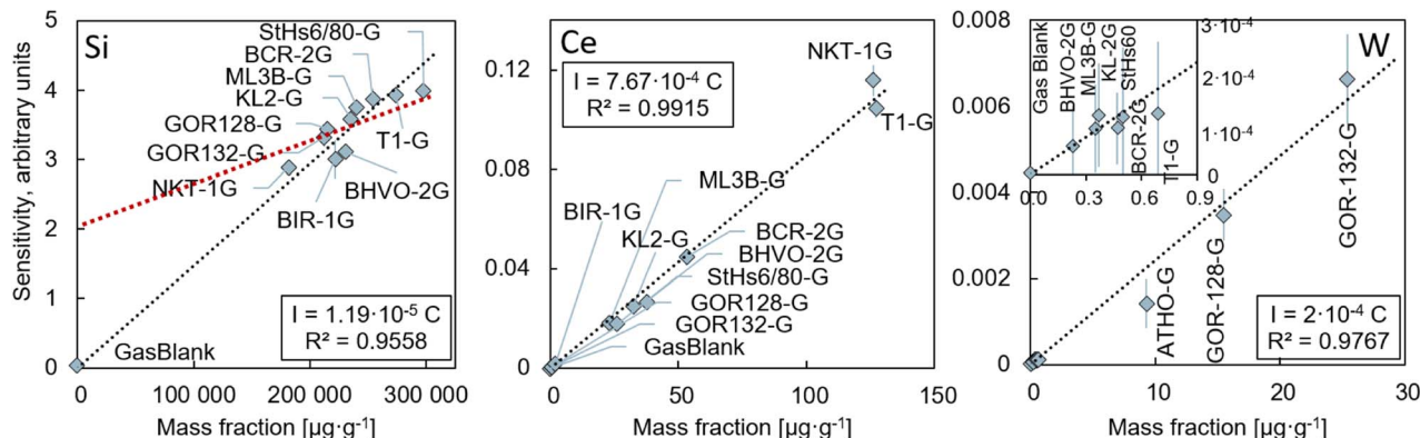
Fig. 1 Calibration lines for LA-ICP-ToF-MS mapping for Si, Ce, and W (left to right). Each point is based on an average of 10 integrated 2D LA-ICP-ToF-MS maps for a GRM (or a gas blank) at the beginning and at the end of the session; error bars correspond to 2SD. Red dashed line – calibration line for Si without forcing it through the origin and not including the gas blank.
