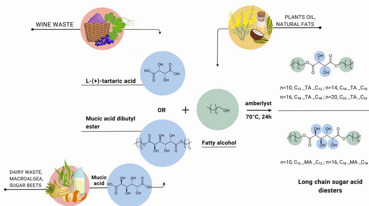
Fig. 1 Scheme of synthesis of long-chain tartaric acid diesters ( C_{12\_TA\_C_{12}} , C_{16\_TA\_C_{16}} , C_{18\_TA\_C_{18}} , and C_{22\_TA\_C_{22}} ) and mucic acid diesters ( C_{12\_MA\_C_{12}} and C_{18\_MA\_C_{18}} ).
