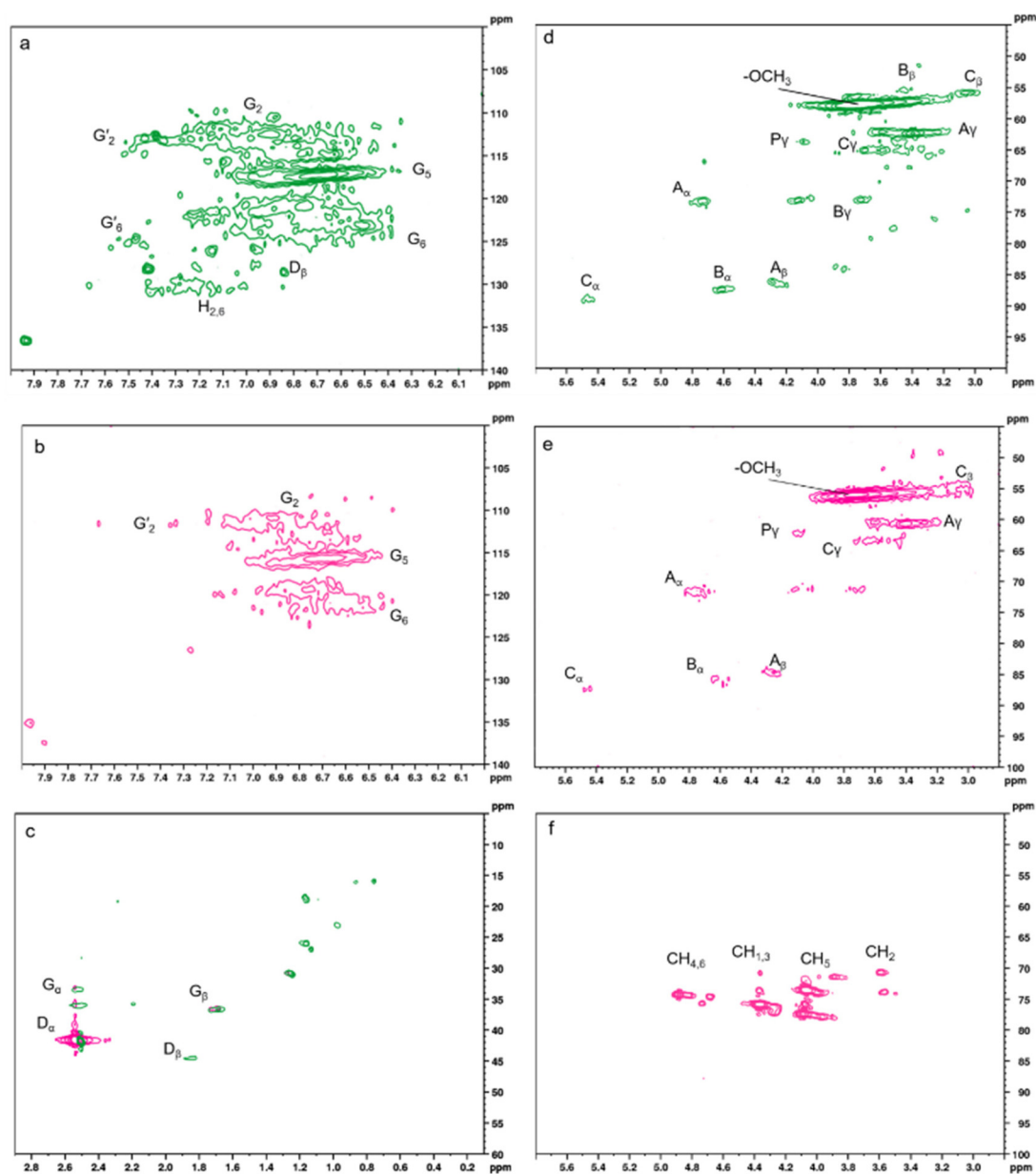
Fig. 5 HSQC NMR spectra (a and d) of KL, (b and e) PK17 in DMSO, (c) aliphatic region of both KL and PK17 in DMSO, and (f) PK17 in D_2O .
