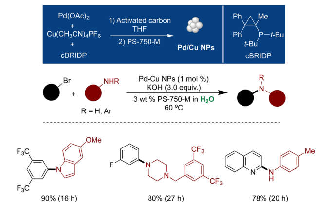
Scheme 30 Bimetallic Cu/Pd NPs for Buchwald–Hartwig aminations in an aqueous micellar medium.
