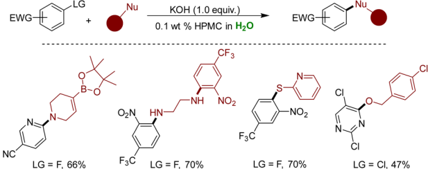
Scheme 41 HPMC enabled nucleophilic aromatic substitution reactions in an aqueous medium.
