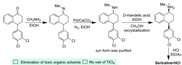
Scheme 4 Greener commercial route for the synthesis of Sertraline (Zolof).
