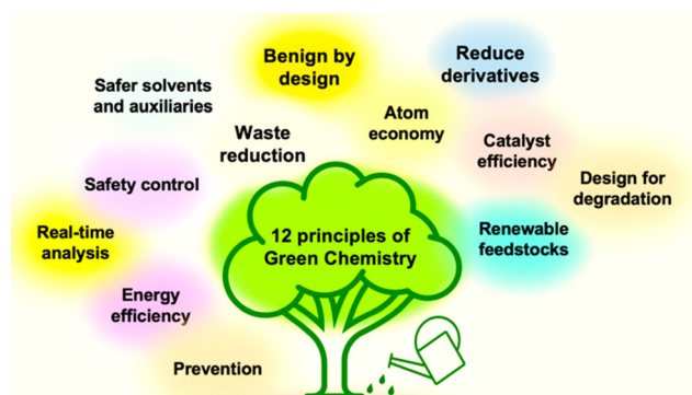
Fig. 1 12 principles of green chemistry.
