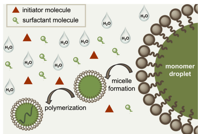
Fig. 5 Mechanism of emulsion polymerization.
