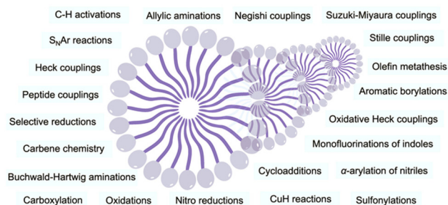
Fig. 3 An overview of organic transformations enabled by micellar catalysis.
