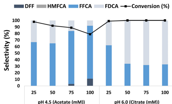
Fig. 4 Effect of buffer (acetate pH 4.5 and citrate pH 6.0) and ionic strength (25, 50, 75, and 100 mM, respectively) in the selectivity and conversion on the oxidation HMF by LacTV-TEMPO system. Reaction condition: HMF (25 mM), TEMPO (0.3 equivalents), LacTV (5 U), reaction time (48 h), 30 °C and 300 rpm.
