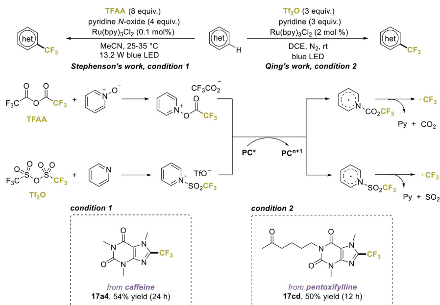
Fig. 48 Photoredox trifluoromethylation of heterocycles with TFAA and \text{Tf}_2\text{O} .
