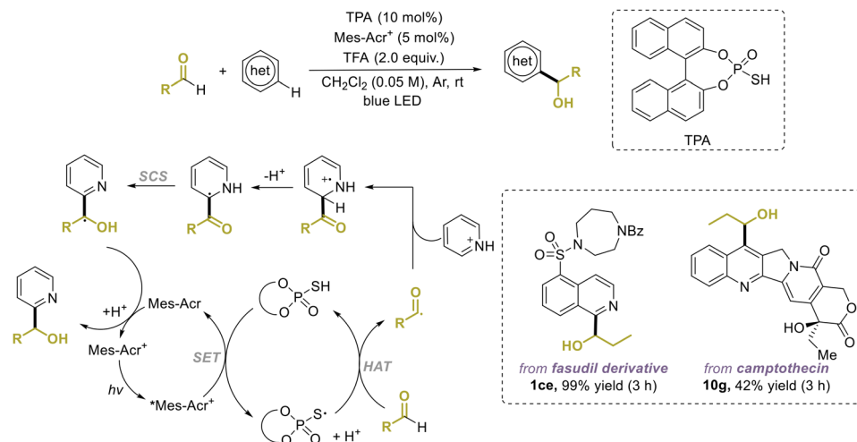
Fig. 37 Photocatalytic Minisci \alpha -hydroxyalkylation with aldehydes.
