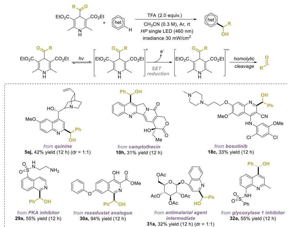
Fig. 38 Photo-mediated Minisci \alpha -hydroxyalkylation with acyl-DHPs.
