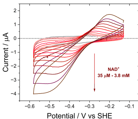
Fig. 4 Activity of Y354S with \text{NAD}^+ , monitored via cyclic voltammetry. \text{NAD}^+ was titrated from 35 \mu\text{M} to 3.8 mM. Experimental conditions: buffer: 50 mM MES, 50 mM TAPS pH 8; scan rate 5 \text{mV s}^{-1} ; electrode Y354S@ITO/PGE; [ \text{NAD}^+ ] indicated on the graph; cell solution purged with argon to remove the contribution to the current from oxygen.
