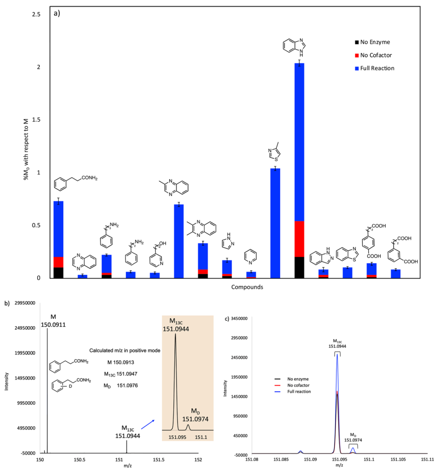
Fig. 3 (a) Plot showing solvent deuterium incorporation in various substrates catalyzed by purified, holo-FDC. Mol% deuterium incorporations (% M_{\text{D}} ) are shown relative to molecular ion (M) peak for each compound. (b) Mass spectrum showing the calculated and experimental M, M_{13\text{C}} and M_{\text{D}} peaks for 3-phenylpropanamide substrate. (c) Mass spectra for 3-phenylpropanamide of the experimental reaction, no enzyme, and no cofactor controls overlayed for comparison.
