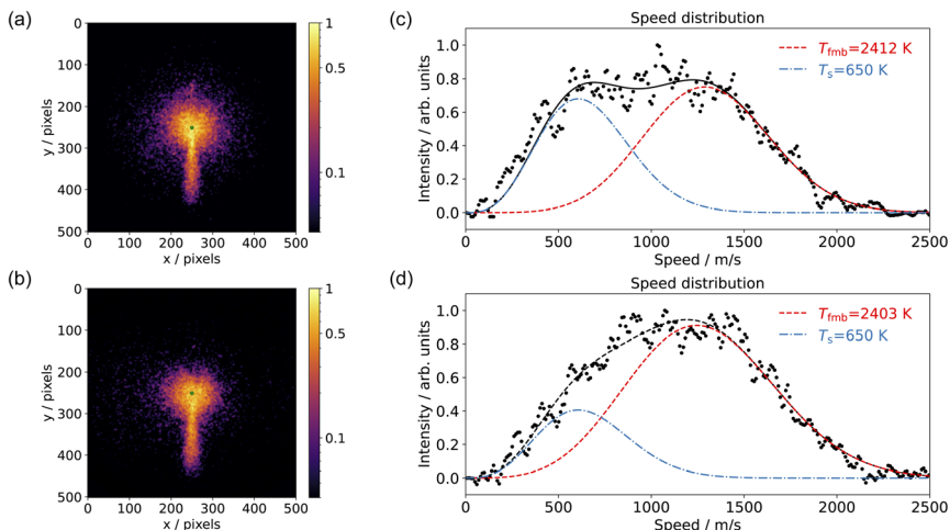
Fig. 4 Comparison of the velocity-map images of CO 2 from CO oxidation on Pd(110) at T_s = 650 K and (a) a pure CO beam with p_{\text{O}_2} = 7.5 \times 10^{-8} mbar; (b) a 10% O 2 in He beam with p_{\text{CO}} = 5 \times 10^{-6} mbar in the scattering chamber. The green dot in (a) and (b) represents the center of the image (zero velocity). (c) and (d) show the corresponding speed distributions (black dots) for CO 2 from (a) and (b), respectively. The speed distribution is fitted (black dashed) with one slow component (blue dashes) and one fast component (red dashes).
