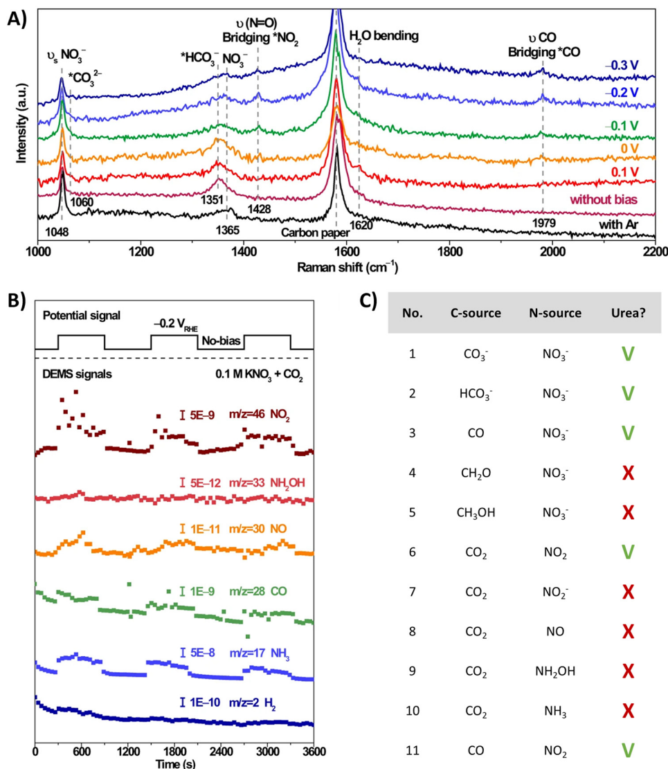
Fig. 16 Mechanistic investigations involving the formation of \text{*O}_2\text{NCO} using the \text{CuWO}_4 catalyst. (A) In situ Raman spectra at different potentials. (B) Online DEMS at -0.2 V vs. RHE. (C) Control experiment with various C- and N-sources. Adapted from ref. 188 (Open Access).
