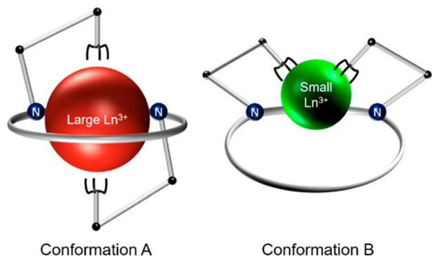
Scheme 2 Depiction of the conformational toggle present in \text{Ln}^{3+} -py-macrodipa and \text{Ln}^{3+} -py 2 -macrodipa complexes. Reproduced with permission from A. Hu, S. N. MacMillan, J. J. Wilson, Macrocyclic Ligands with an Unprecedented Size-Selectivity Pattern for the Lanthanide Ions , J. Am. Chem. Soc. 2020, 142 , 13500–13506. Copyright 2020 American Chemical Society.
