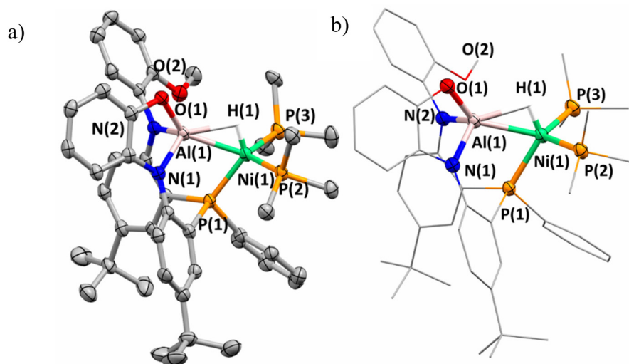
Fig. 3 (a) Solid-state structure of anionic portion of complex 3 . Cation and hydrogen atoms on ligands are excluded for clarity. (b) Mixed wire-frame/ellipsoid structure of complex 3 shown for clarity.
