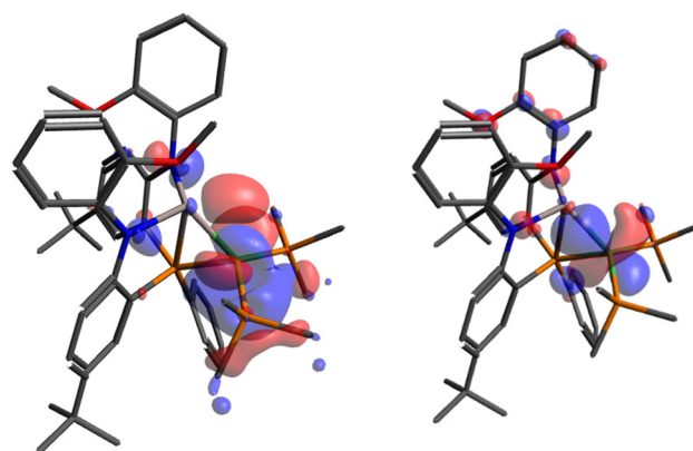
Fig. 5 Pictorial representation of HOMO (left) and HOMO (–6) (right) of 2-(PMe 3 ) 2 . Isosurface value set to 0.03 \text{ e} \text{ \AA}^{-3} . Hydrogen atoms are omitted for clarity.
