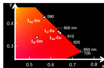
Fig. 3 CIE 1931 x, y chromaticity coordinates as a function of the emission wavelengths for 1 Si -Sm , 1 Ge -Sm , 1 Si -Eu and 1 Ge -Eu .
