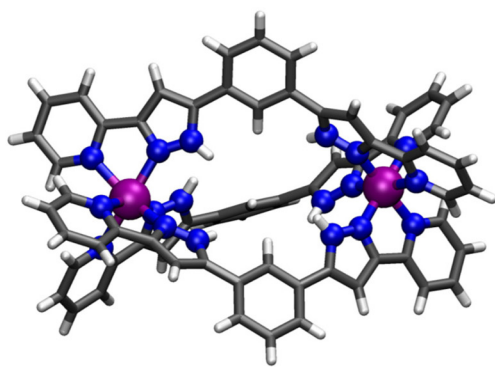
Fig. 1 (Left) The [\text{Fe}_2(\text{L}_1)_3]^{4+} system ( \text{L}_1 = 1,3\text{-bis}(3\text{-(pyridin-2-yl)-1H-pyrazol-5-yl})\text{benzene} ) and (right) schematic depiction of the subunit [\text{Fe}(\text{L}_2^{\text{R}})_3]^{2+} ( \text{L}_2 = 3\text{-(2-pyridyl)pyrazole} ), showing the R positions used to screen for ligand functionalization. Blue for N, purple for Fe, grey for C and white for H.
