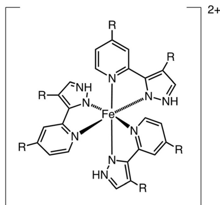
Fig. 1 (Left) The [\text{Fe}_2(\text{L}_1)_3]^{4+} system ( \text{L}_1 = 1,3\text{-bis}(3\text{-(pyridin-2-yl)-1H-pyrazol-5-yl})\text{benzene} ) and (right) schematic depiction of the subunit [\text{Fe}(\text{L}_2^{\text{R}})_3]^{2+} ( \text{L}_2 = 3\text{-(2-pyridyl)pyrazole} ), showing the R positions used to screen for ligand functionalization. Blue for N, purple for Fe, grey for C and white for H.
