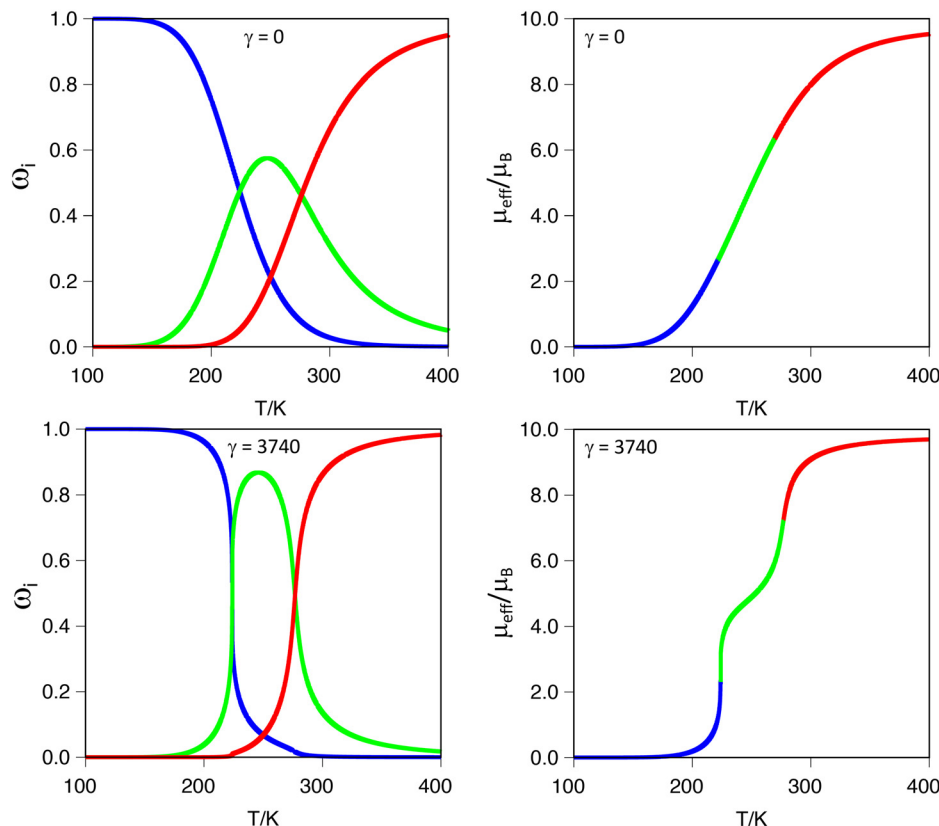
Fig. 4 (Left) Spin state populations ( \omega_i ) for the [\text{Fe}_2(\text{L}_1)_3]@\text{Cl} systems with \gamma = 0 (top) and \gamma = 3740 (bottom): i = [\text{LS-LS}] (blue), [\text{HS-LS}] (green) and [\text{HS-HS}] (red) populations. (Right) Estimation of the magnetic moment computed from the corresponding spin-state populations. \gamma in \text{J mol}^{-1} .
