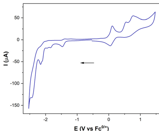
Fig. 7 CV of complex 23 , obtained from 10^{-3} \text{ M} solutions in MeCN containing [\text{nBu}_4\text{N}]\text{PF}_6 10^{-1} \text{ M} as the supporting electrolyte, recorded at 25^\circ \text{C} . Counter-electrode: Pt; working electrode: vitreous carbon; potentials given in V vs. \text{Fc}^+/\text{Fc} ; scan rate: 100 \text{ mV s}^{-1} .
