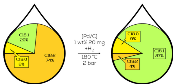
Fig. 20 Composition of the C18 fatty acid fraction in the selective hydrogenation of sunflower oil as performed by Romanenko. 121
