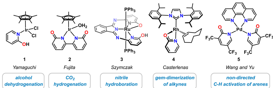
Scheme 2 Selected examples of noble metal pyridonate catalysts for hydrofunctionalizations.
