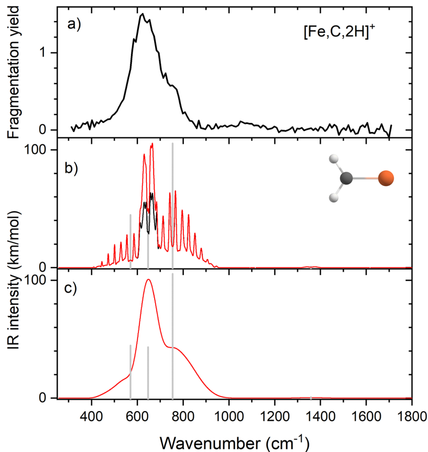
Fig. 2 (a) Experimental IRMPD spectrum of [\text{Fe,C,2H}]^+ ; (b) harmonic stick spectrum of the \text{FeCH}_2^+ ( {}^4\text{B}_1 ) structure at the CCSD/def2-TZVPPD level and rovibrational simulations using the original IR intensity for the Fe–C stretch mode at 43 \text{ km mol}^{-1} (black) and with a double value (red); (c) same as (b) but convolved with a 9% FWHM Gaussian lineshape function to simulate broadening effects.
