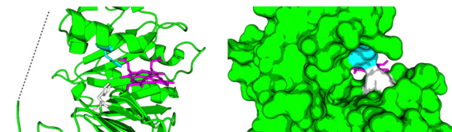
Fig. 7 Large cavity of HemS. It is split into two smaller cavities by a central pair of phenylalanine residues, F104 (white) and F199 (cyan). In one cavity, heme binds. In the other, Relibase + identified a possible NADH-binding site. A dashed line has been included to represent the missing loop region from the crystal structure (2J0P).
