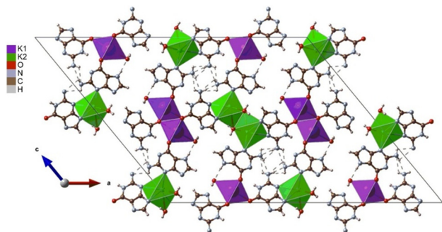
Fig. 3 K-guanine ( K^+ \cdot C_5H_3N_5O^- \cdot H_2O ) displays 2 types of edge-sharing polyhedral chains of the cations in b -direction. K1 (violet) entirely coordinates to oxygen, originating from water and guanine, while K2 (green) interacts with water and organic nitrogen (O6, N3, N9). 34
