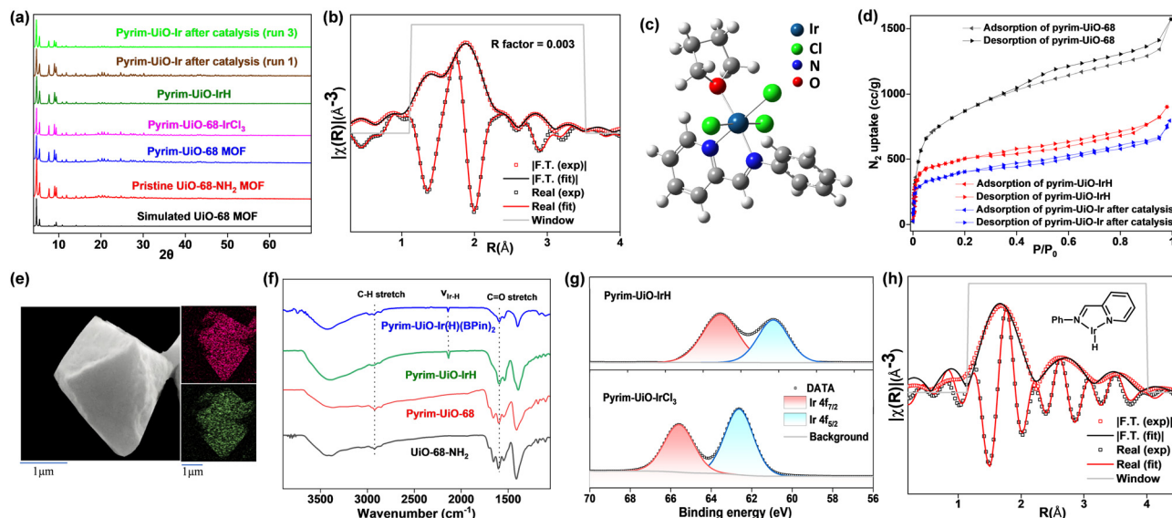
Fig. 2 (a) PXRD patterns of simulated UiO-68 MOF (black), pristine UiO-68-NH 2 MOF (red), pyrim-UiO-68 MOF (blue), pyrim-UiO-68-Cl 3 (magenta), pyrim-UiO-IrH (olive), pyrim-UiO-Ir after run 1 (brown) and pyrim-UiO-Ir after run 3 (green). (b) EXAFS spectra (red and black hollow squares) and fits (red and black solid lines) of pyrim-UiO-IrCl 3 in the R space from 1.15–3.5 Å. (c) DFT optimised structure of (pyrim)IrCl 3 (THF) molecule. (d) BET nitrogen sorption isotherms of pyrim-UiO-68 (black), pyrim-UiO-IrH (red) and pyrim-UiO-Ir after catalysis (blue) measured at 77 K. (e) SEM image of a pyrim-UiO-IrH particle along with elemental mapping of Zr and Ir. (f) IR (KBr) spectrum of UiO-68-NH 2 (black), pyrim-UiO-68 MOF (red), pyrim-UiO-IrH (green) and pyrim-UiO-IrH(BPin) 2 (blue). (g) Ir 4f XPS spectra of pyrim-UiO-IrCl 3 and pyrim-UiO-IrH. (h) EXAFS spectra (red and black hollow squares) and fits (red and black solid lines) of pyrim-UiO-IrH in the R space from 1.15–4.0 Å.
