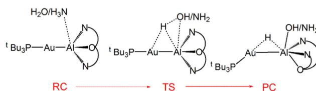
Scheme 10 Sketched structures of the stationary points along the reaction profile calculated for the O–H/N–H bond activation of H_2O/NH_3 with the Au–Al bond. RC = reactant complex, TS = transition state, PC = product complex.
