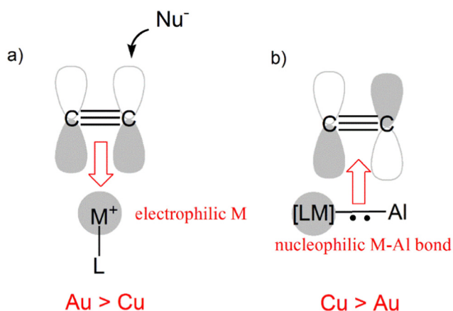
Scheme 9 (a) Electrophilic behaviour of [LM]^+ ( M = Cu, Au ) complexes for alkyne activation (Au more efficient than Cu); (b) nucleophilic behaviour of the M–Al ( M = Cu, Au ) bond in coinage metal–aluminyl complexes towards alkynes (Cu more efficient than Au).
