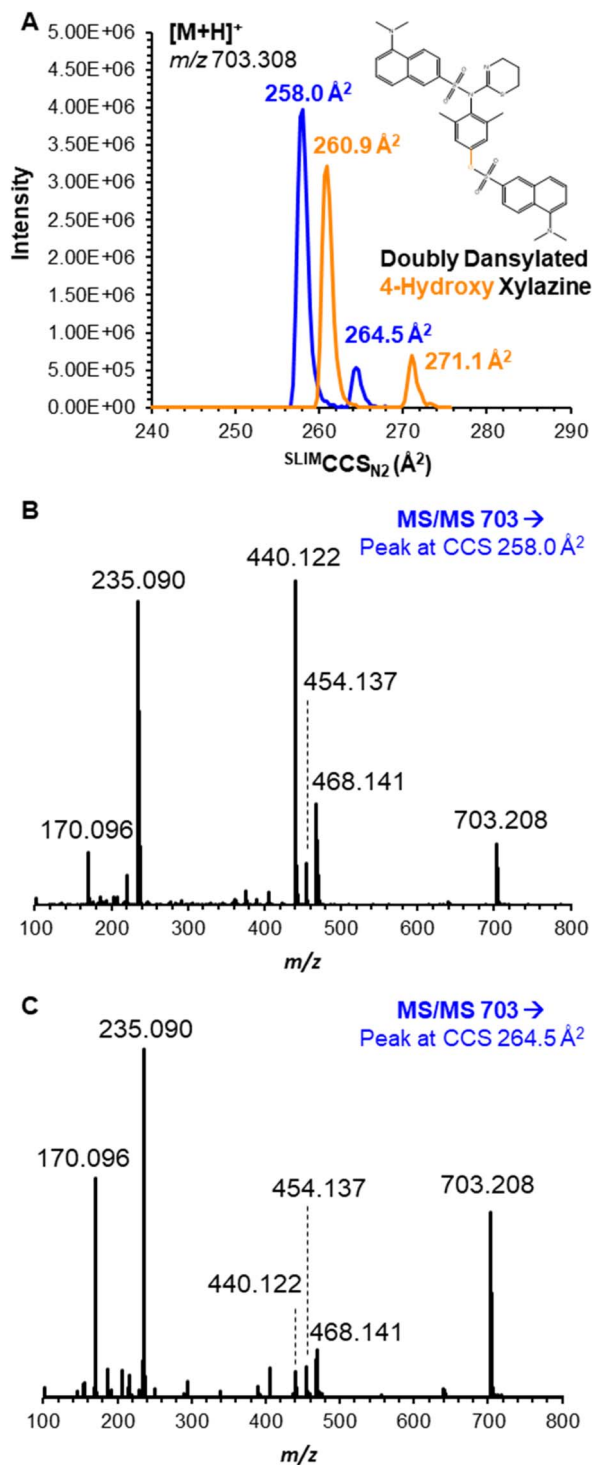
Fig. 3 (A) Ion mobilogram for 3-hydroxy and 4-hydroxy xylazine as the protonated doubly dansylated products at m/z 703. Each individual mobility peak, at (B) CCS 258.0 and (C) CCS 264.5 \text{\AA}^2 , was subjected to mobility-aligned fragmentation (MAF), for which their spectra are shown above.
