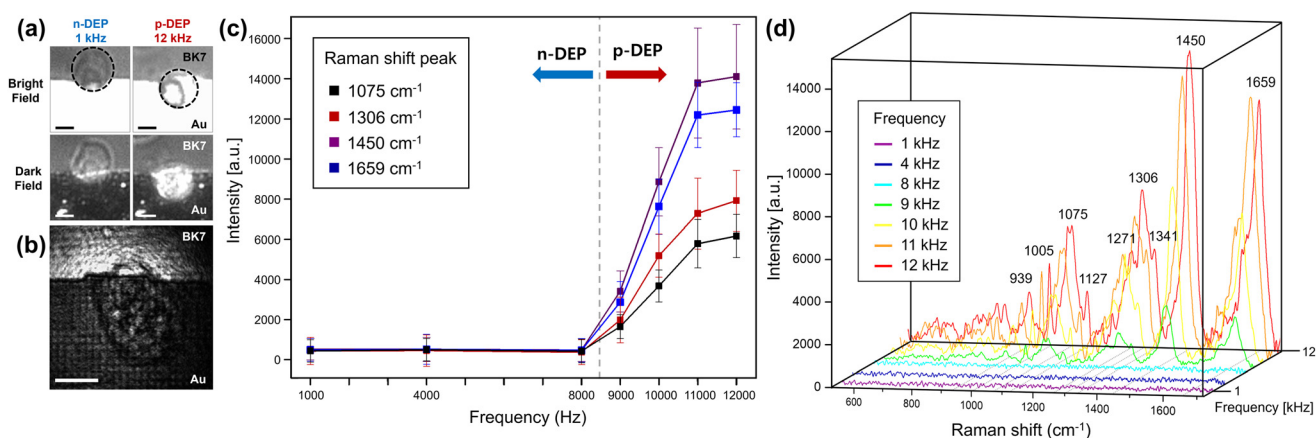
Fig. 5 (a) An optical image of a trapped U-87 MG cell in the bright-field and the dark-field (scale bar: 5\text{ }\mu\text{m} ) captured for the electrode with nanohole arrays and the BK7 glass substrate. (b) Scatter image of a positive trapped U-87 MG cell (scale bar: 5\text{ }\mu\text{m} ). (c) Raman peak intensity of a U-87 MG cell placed on gold nanohole arrays at different DEP frequencies ( n = 10 ). (d) Raman spectra of a U-87 MG cell on gold nanohole arrays at different DEP frequencies. The frequency increases along the z-axis from 1 to 12 kHz.
