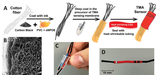
Fig. 4 (A) The process of preparing a home-made TMA sensor for vaginosis analysis. (B) A SEM cross-section image of the membrane coated TMA sensor (scale bar is 50 \mu m). (C and D) Photographs of the sensor depicting its portability and size. 102 Copyright 2023, MDPI.
