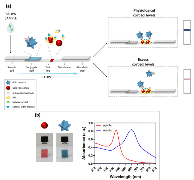
Fig. 12 Design and working principle of the dual-color plasmonic LFIA device; (a) scheme of the proposed POC system, based on the combination of gold nanospheres (AuNPs) and nanostars (AuNSs); (b) the bottom panel displays the plasmonic properties of the two types of gold nanoparticles employed. Reproduced from ref. 92 with permission from Royal Society of Chemistry, copyright 2023.
