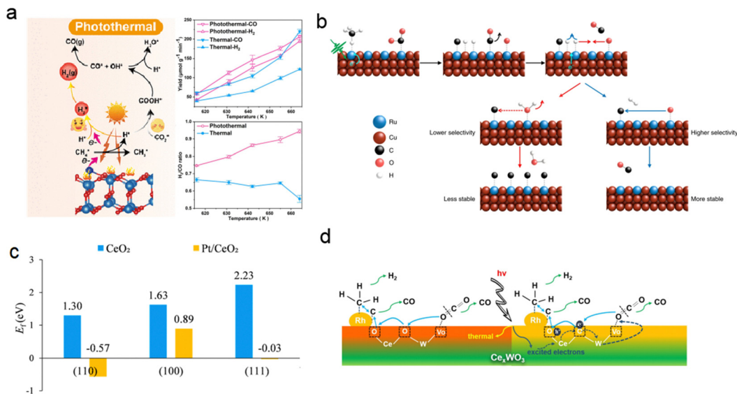
Fig. 15 (a) Schematic and DRM performance of the \text{Ni}/\text{Ga}_2\text{O}_3 catalyst. 129 (b) Schematic of enhanced selectivity and stability in Cu–Ru surface alloys. 130 (c) Oxygen vacancy formation energy of the Pt/CeO _2 catalyst. 131 (d) Schematic diagram for the light-driven DRM reaction over the Rh/Ce _x WO _3 catalyst. 3
