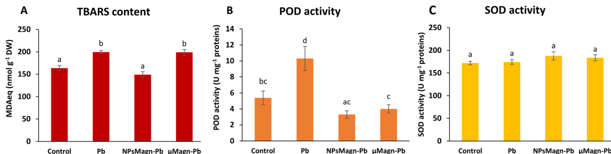
Fig. 3 Lipid peroxidation and antioxidant activities measured in the leaves of sunflower plants after 90 days of growth on control soil or containing Pb, NPsMgn-Pb or \mu Mgn-Pb. (A) TBARS content (nmol MDAeq per g DW); (B) POD activity (U mg per protein); and (C) SOD activity (U mg per protein). Data represent the mean \pm SEM ( n = 6 ). Different letters above the bars indicate significant differences ( p < 0.05 ).
