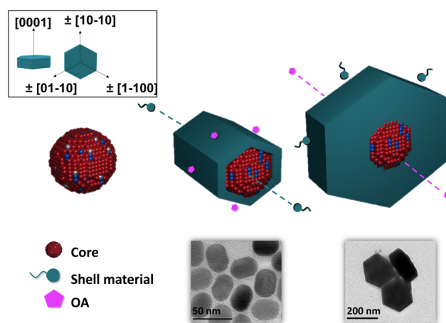
Fig. 2 Proposed mechanism of epitaxial growth of NaLnF 4 shells around the NaYbF 4 :Tm(0.5%)Fe(5%) core.
