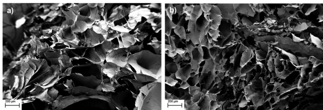
Fig. 1 SEM images of (a) 2 wt% and (b) 4 wt% chitosan scaffolds. 50 \times magnification, scale bars 200 \mu m.
