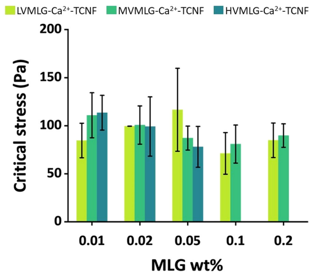
Fig. 7 Wet mechanical properties of self-standing MLG–Ca 2+ –TCNF hydrogel films. Critical stress values of the matrices with LV-, MV-, and HVMLG in 0.01–0.2 wt% concentrations. Standard deviations from at least five replicate measurements are shown.
