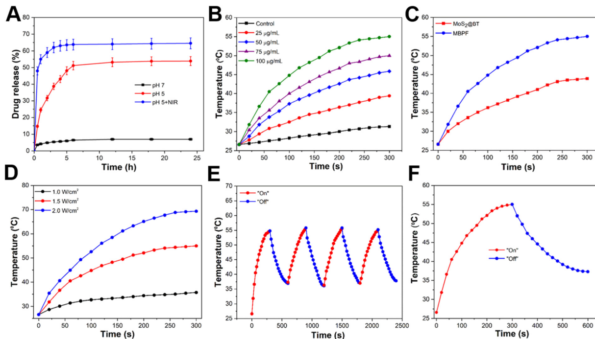
Fig. 3 (A) pH and NIR-based gemcitabine release from MBPF CSNPs. (B) Temperature rise curves of distilled water (control) and MBPF CSNPs under changing concentrations ( 0\text{--}100\text{ }\mu\text{g mL}^{-1} ) when exposed to NIR laser irradiation ( 808\text{ nm} , 1.5\text{ W cm}^{-2} , 5\text{ min} ). (C) Temperature increase curves of \text{MoS}_2\text{@BT} and MBPF CSNPs ( 100\text{ }\mu\text{g mL}^{-1} of concentration) with NIR irradiation. (D) Temperature increase of 100\text{ }\mu\text{g mL}^{-1} of MBPF CSNPs with NIR irradiation for 300\text{ s} at different power densities. (E) Four and (F) single rounds of NIR irradiation with on/off cycling for 600\text{ s} intervals.
