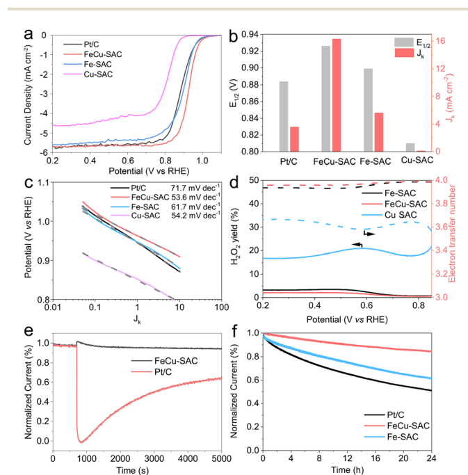
Fig. 3 ORR performance of FeCu-SAC, Fe-SAC, Cu-SAC and commercial Pt/C. (a) LSV curves. (b) Half-wave potential and kinetic current density at 0.9 V. (c) Tafel slope of FeCu-SAC, Fe-SAC, Cu-SAC and commercial Pt/C. (d) H 2 O 2 yield and calculated electron transfer tested by RRDE. (e) Methanol tolerance of FeCu-SAC and commercial Pt/C. (f) Amperometric i - t curves of FeCu-SAC, Fe-SAC and commercial Pt/C.
