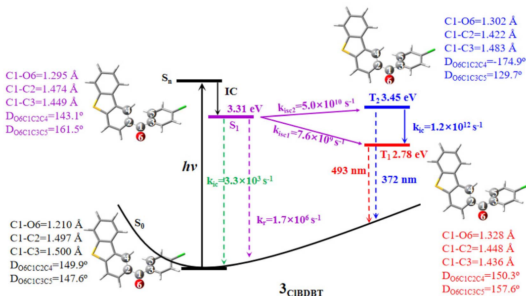
Fig. 3 The adiabatic energy levels, radiative ( k_{\text{r}} ) and nonradiative ( k_{\text{ic}} and k_{\text{isc}} ) rates, as well as T 1 and T 2 emission wavelengths for 3_{\text{CIBDBT}} . The ground state energy (−1660.75414666 a.u.) of 3_{\text{CIBDBT}} is set as the reference at the CC2/cc-pVDZ level. The geometrical parameters for some important bonds and dihedral angles are also shown.
