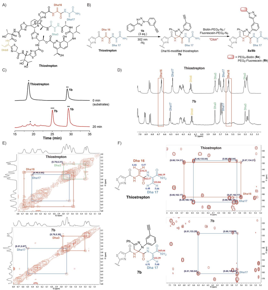
Fig. 3 Site-selective labelling of thiostrepton via light-initiated 1,3-dipolar cycloaddition of Dha and tetrazole 1b . (A) Chemical structure of thiostrepton. (B) Two-step reaction for site-specific labelling of Dha16 on thiostrepton. (C) HPLC analysis of the reaction mixture of thiostrepton and tetrazole 1b at 0 min (top) and 20 min (bottom). (D) ^1\text{H} NMR spectra of thiostrepton and Dha16-labelled product 7b . Chemical shifts of signals from the \text{C}(\text{sp}^2)\text{-H} of Dha3, Dha16, Dha17, and Dhb8 are assigned. (E) 2D-NMR spectra ( ^1\text{H}\text{-}^1\text{H} COSY) of thiostrepton and 7b , which show ^1\text{H}\text{-}^1\text{H} couplings in Dha16 and Dha17. (F) 2D-NMR spectra ( ^1\text{H}\text{-}^{13}\text{C} HMBC) of thiostrepton and 7b . Long range ^1\text{H}\text{-}^{13}\text{C} couplings via a \text{H}\text{-C}\text{-C}\text{-C} path are measured and assigned.
