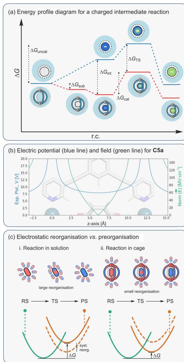
Fig. 13 (a) Energy profile diagram for a reaction with a charged intermediate; (b) electric potential (blue line), V , and field (green line), E , exemplified for a [\text{Pd}_2\text{L}_4]^{4+} cage; (c) electrostatic TS stabilisation via a preorganised microenvironment.
