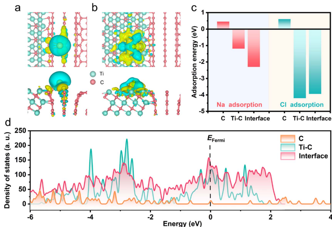
Fig. 7 Differences in charge densities for Na (a) and Cl (b) adsorbed by the interface of CNF and Ti_3C_2T_x . (c) Adsorption energy for Na and Cl adsorption of CNF, Ti_3C_2T_x , and Ti_3C_2T_x/CNF . (d) DOS spectra of CNF, Ti_3C_2T_x , and Ti_3C_2T_x/CNF .
