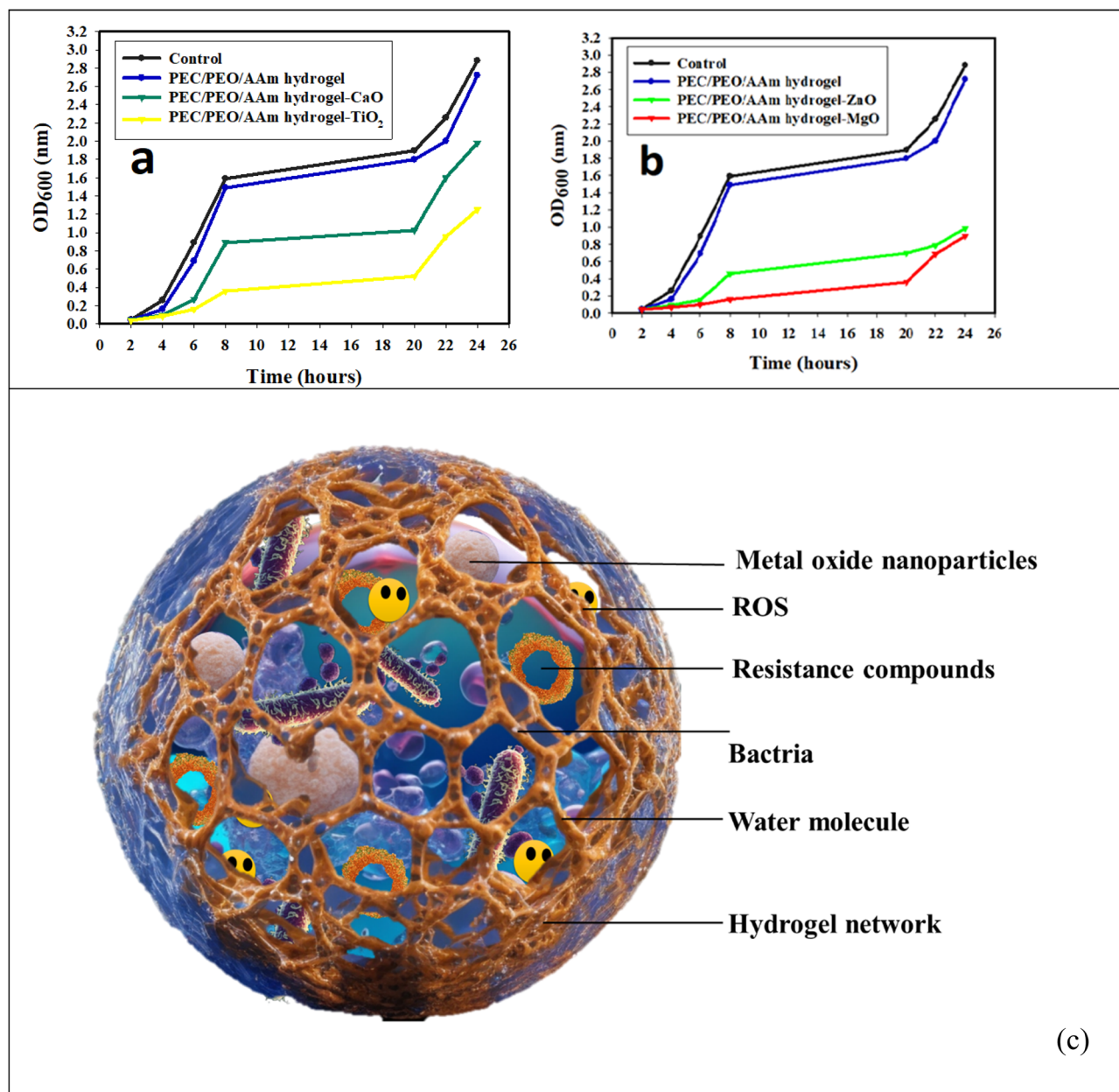
Fig. 9 Impact of PEC/PEO/AAM hydrogel, modified with CaO and TiO 2 (a), and PEC/PEO/AAM hydrogel, modified with ZnO and MgO (b), on S. aureus Growth curve and (c) synergistic antibacterial mechanism of nanoparticles.
