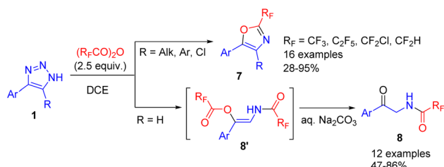
Scheme 8 Synthesis of fluoroalkylated oxazoles and 2-acylamino-ketones from NH-1,2,3-triazoles with fluoroalkylated acid anhydrides.
