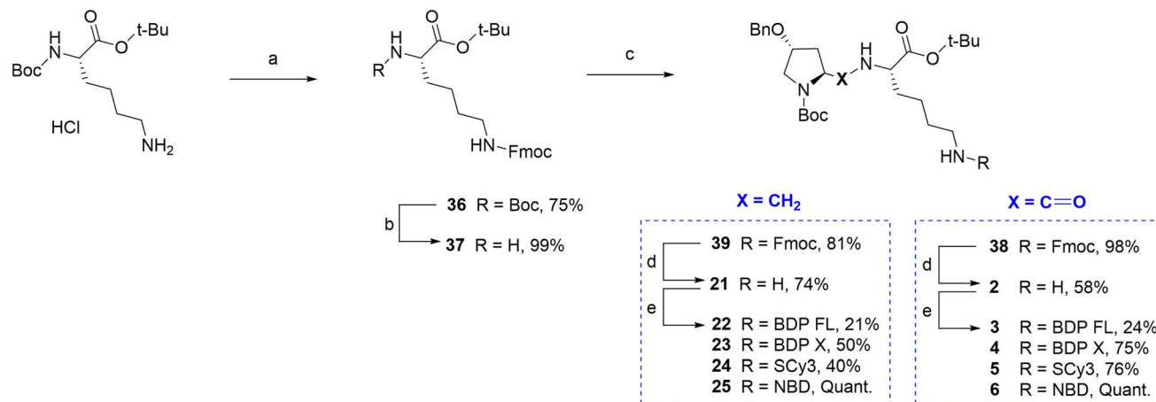
Scheme 4 Synthesis of fluorescent conjugates 3–6 , 22–25 . Reagents and conditions: (a) 10% \text{NaHCO}_3 aqueous solution, THF, Fmoc-NHS, 0^\circ\text{C} , rt, overnight; (b) 4 N HCl in 1,4-dioxane, \text{N}_2 , 0^\circ\text{C} , rt, 75 min; (c) MeOH, (4R)-benzyloxy-(2S)-formyl-pyrrolidine-1-carboxylic acid tert -butyl ester, \text{NaBH}_3\text{CN} , \text{CH}_3\text{COOH} , rt, 3 h; (d) dry DMF, \text{N}_2 , diethylamine, rt, 60 min; (e) dry DMF ( 3 , 4 , 5 , 22 )/acetonitrile ( 23 , 24 ), \text{N}_2 , triethylamine, NHS-activated fluorophore, rt, 2 h ( 3 )/18 h ( 4 )/20 h ( 5 )/3 days ( 22 )/1 h ( 23 )/45 min ( 24 ) or MeOH, \text{N}_2 , \text{NaHCO}_3 , NBD chloride, rt, overnight ( 6 )/2 days ( 25 ).
