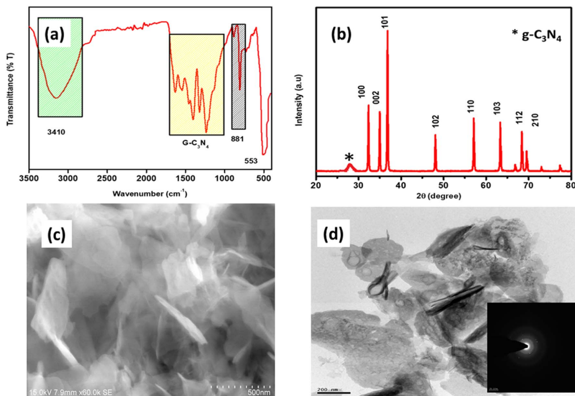
Fig. 1 (a) The FTIR spectrum, (b) XRD pattern, (c) SEM, and (d) HRTEM analysis of the g-C 3 N 4 @ZnO nanocomposite.
