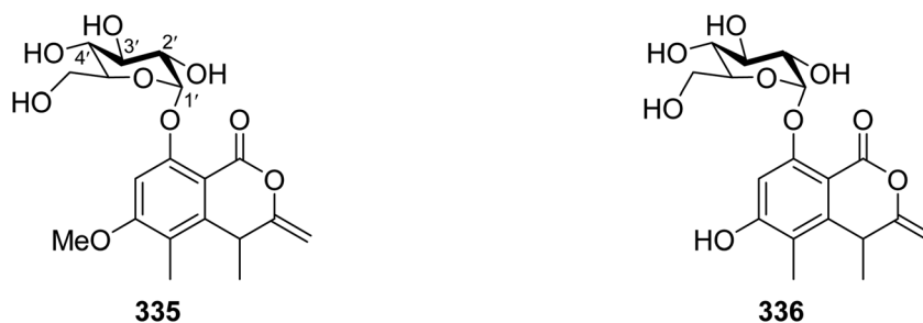
Fig. 49 Chemical structures of 335–336.
