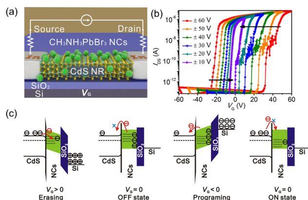
Fig. 13 (a) Schematic device structure of \text{MAPbBr}_3 NCs/CdS NR memory transistor. (b) Electrical transfer characteristics at V_{DS} = 1 V of the device recorded after every sweeping cycle. (c) Energy band diagrams of the device during the charge storage process. Reproduced with permission. 207 Copyright © 2019, American Chemical Society.
