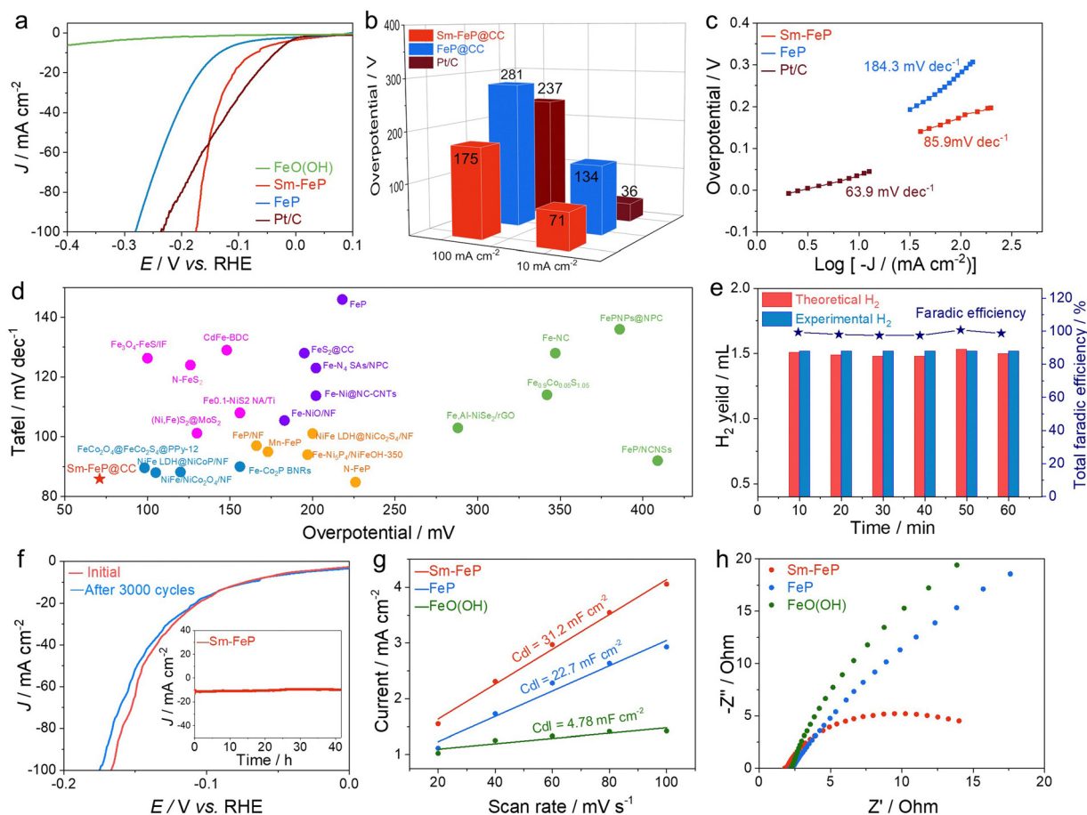
Fig. 4 Comparison of the HER activity of Sm-FeP@CC with other samples in 1 M KOH solution: (a) HER polarization curves; (b) overpotentials at 10 \text{mA cm}^{-2} and 100 \text{mA cm}^{-2} ; (c) Tafel plots derived from (a); (d) HER performance comparison of Sm-FeP@CC with other recently reported Fe-based catalysts; (e) the \text{H}_2 yield and faradaic efficiency of Sm-FeP@CC for the HER; (f) HER polarization curves of Sm-FeP@CC before and after 3000 cycles of CV, where the inset shows the i - t curve of Sm-FeP@CC; (g) C_{dl} values and (h) EIS Nyquist plots of the catalysts.
