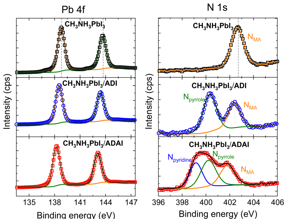
Fig. 10 Pb 4f and N 1s core level XPS spectra of bare \text{CH}_3\text{NH}_3\text{PbI}_3 and \text{CH}_3\text{NH}_3\text{PbI}_3 coated with ADI and ADAl.
