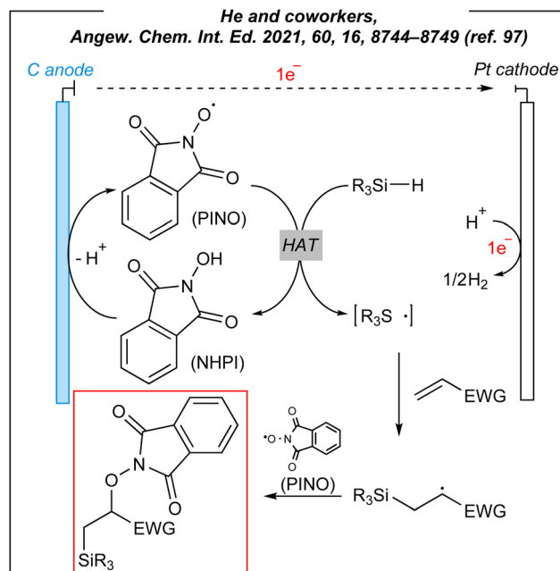
Fig. 11 Plausible mechanism for the 1,2-silylfunctionalization.
