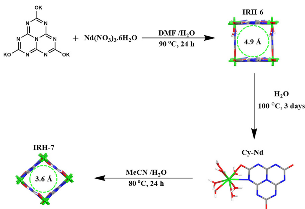
Fig. 1 Synthesis routes of IRH-6, Cy-Nd and IRH-7.
