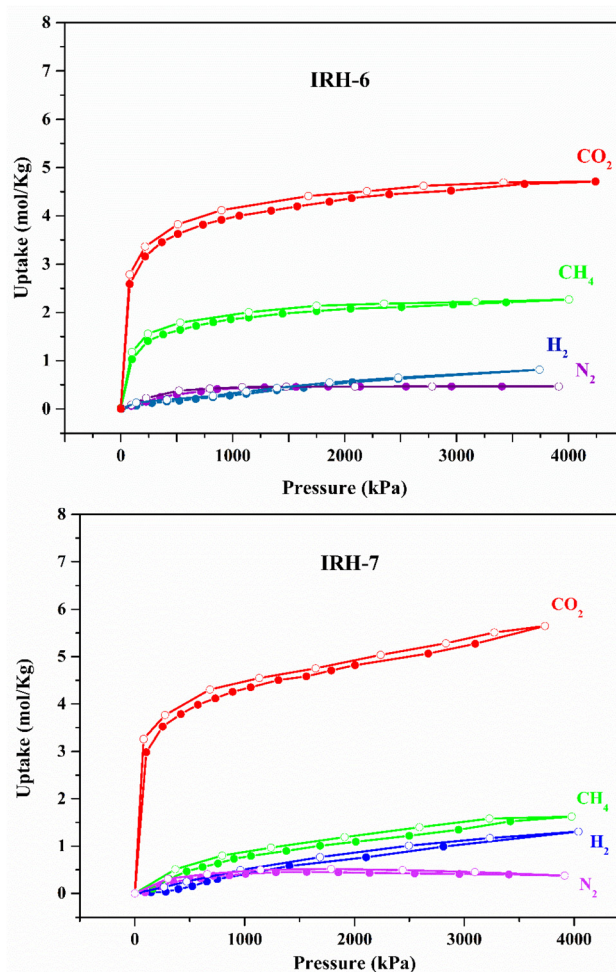
Fig. 4 Experimental adsorption isotherms of \text{CO}_2 , \text{CH}_4 , \text{N}_2 , and \text{H}_2 at 298 K for IRH-6 and IRH-7.
