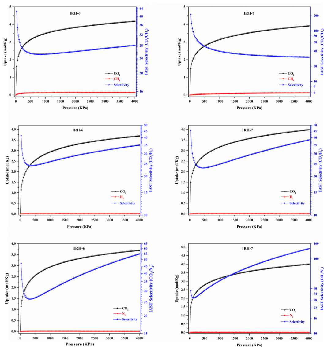
Fig. 6 IAST adsorption isotherms and \text{CO}_2 selectivity of IRHs 6 and 7 for the \text{CO}_2/\text{CH}_4 (50 : 50), \text{CO}_2/\text{N}_2 (15 : 85), and \text{CO}_2/\text{H}_2 (15 : 85) mixtures.
