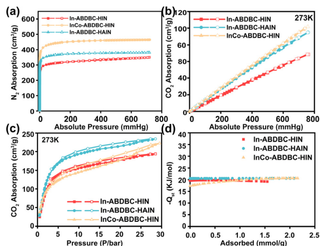
Fig. 3 (a) N 2 adsorption and desorption isotherms at 77 K, (b) low-pressure CO 2 adsorption isotherms at 273 K and (c) high-pressure CO 2 adsorption isotherms at 273 K for In-ABDBC-HIN, InCo-ABDBC-HIN, and In-ABDBC-HAIN. (d) Isotheric heat of adsorption (Q st ).
